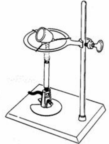
ring stand (base and metal stick); iron ring (ring clamped to metal stick); crucible; clay triangle (almost hidden – just see wires); bunsen burner
